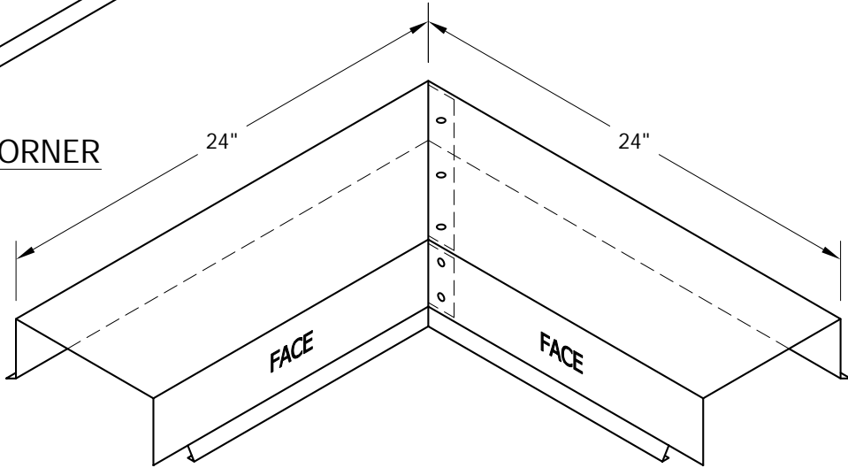
INSIDE CORNER
