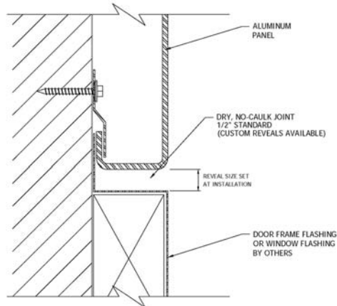
Dry Seal Joint Detail
