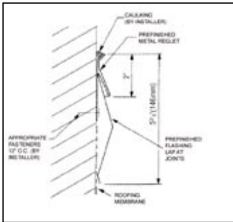
Concealed-Mount CMR 575
