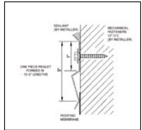
Surface-Mount SR 50
